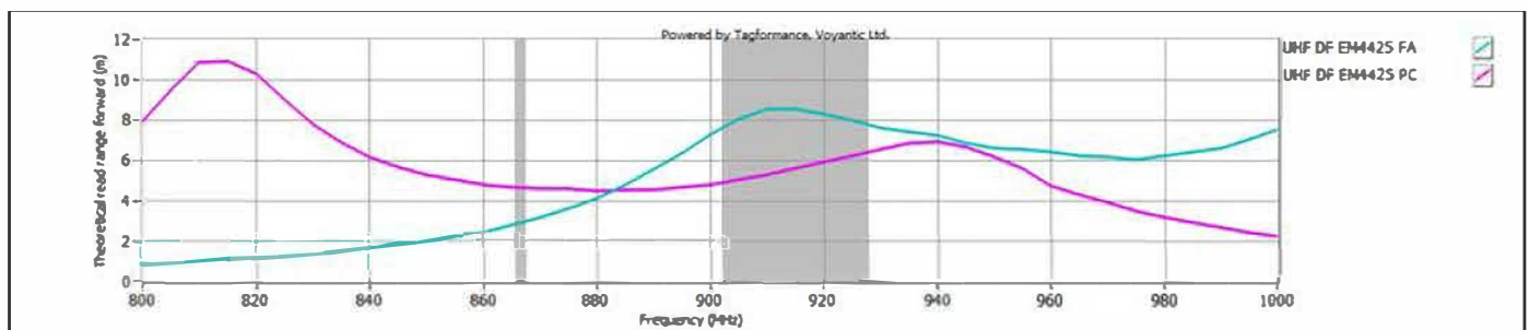
PID DUAL FREQUENCY - RF performance(EM4425)
