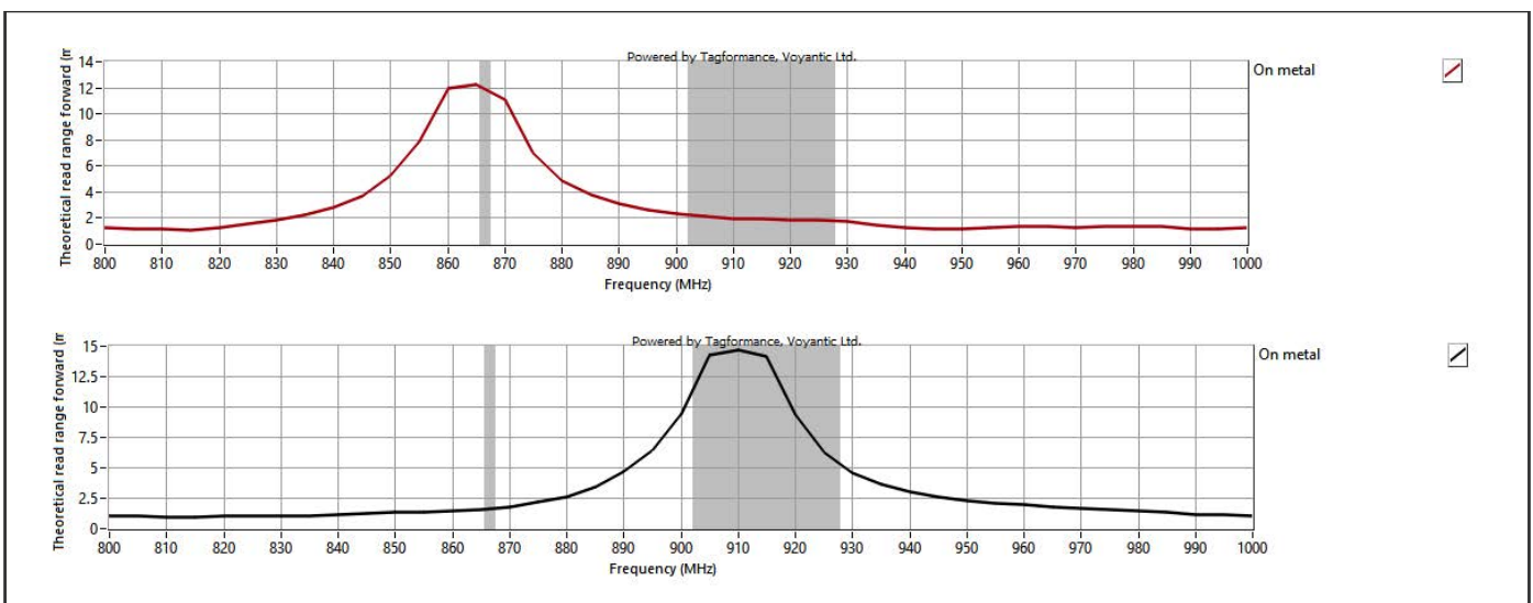
UNI 7030 - RF performance
