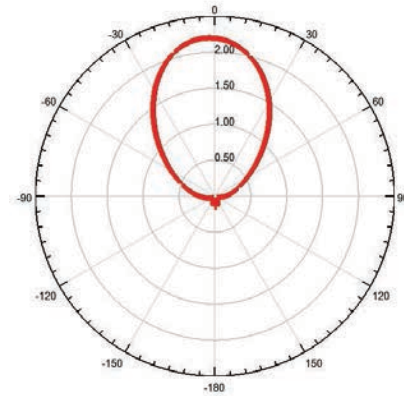
Raditation Pattern 2
