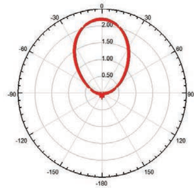
Raditation Pattern 1
